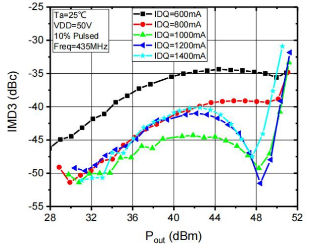
Two Tone IMD3 vs Pout @Idq's
