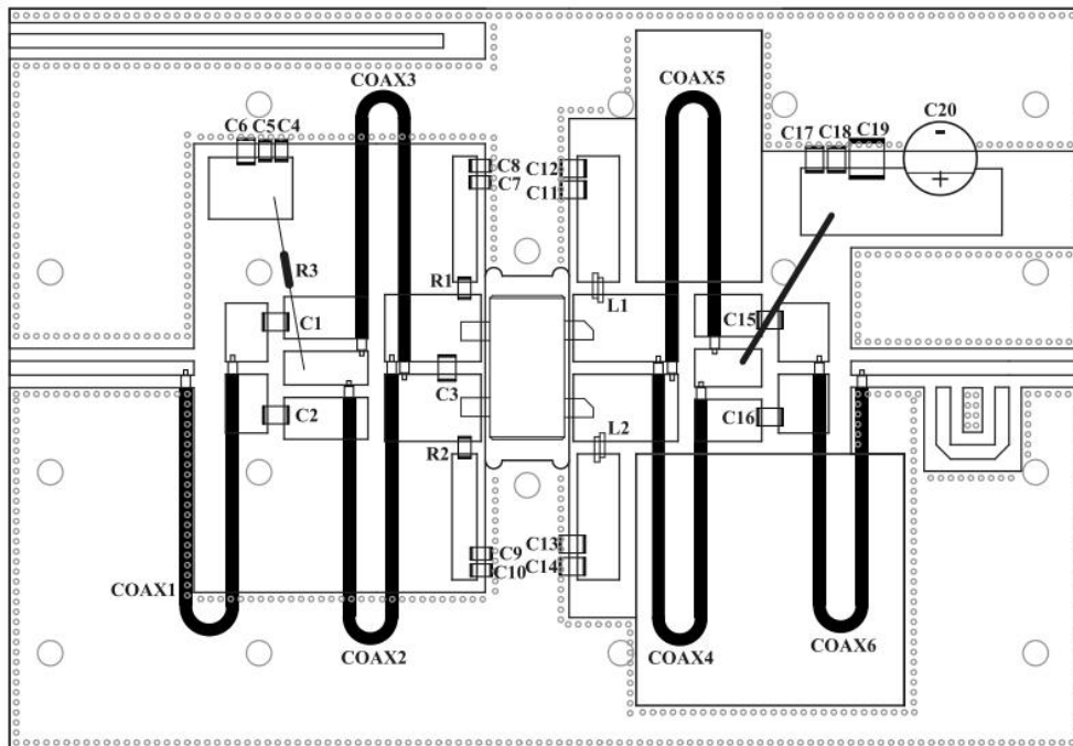
EVB Layout
